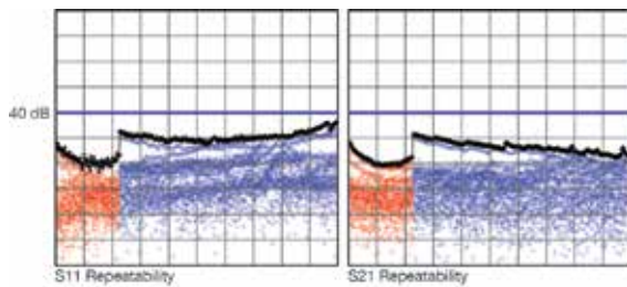
Repeatability for XT982GL01 7mm automated tuners.
