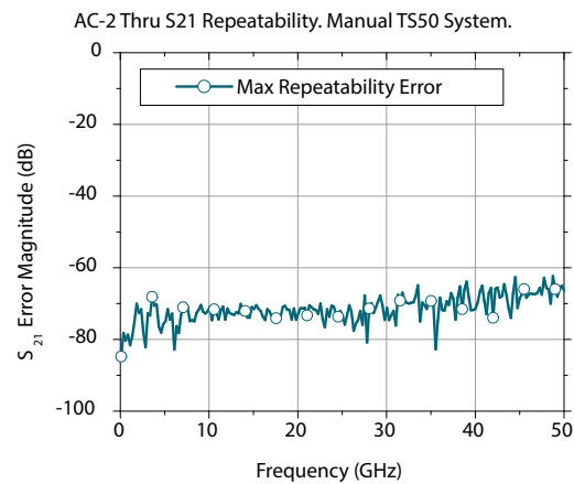
The maximal probe contact repeatability error of the calibrate S 21 -parameter of the AC-2 thru standard by T50 probes. Manual probe system TS50.
